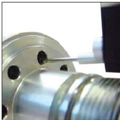
Measurement in small bores
