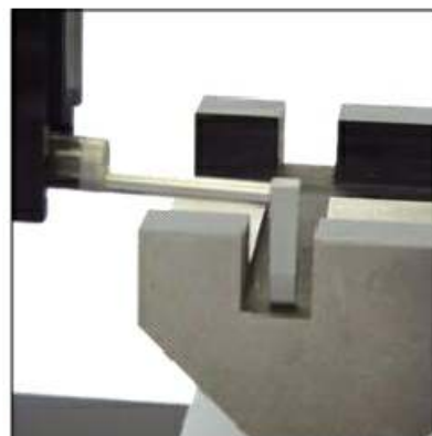
Checking in a recess using an appropriate probe
